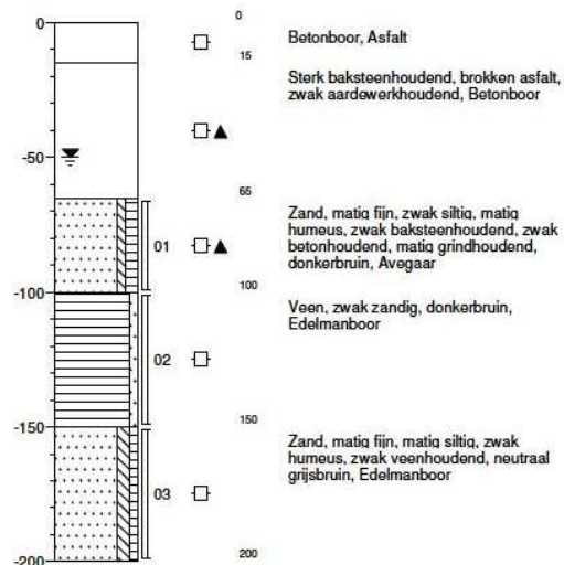
Boring: 204
