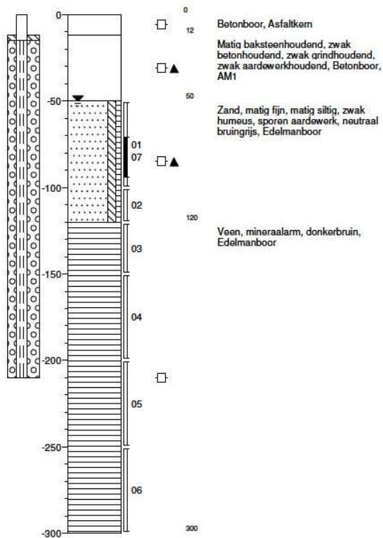
Boring: 203
