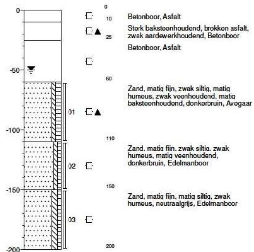
Boring: 202
