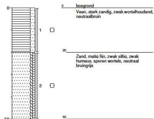
Boring: 10
