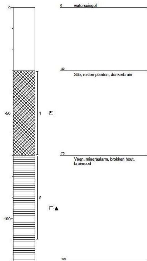
Boring: S07
