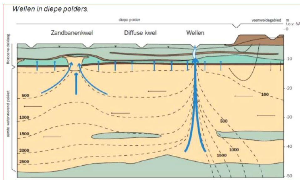
Figuur 14: wellen in diepe polders (Arcadis, 2016)
